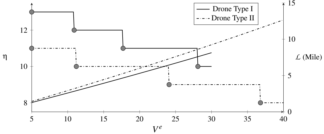
Figure 9: Optimal Number of Drones and Optimal Length of the E-line for Different Drone Types
