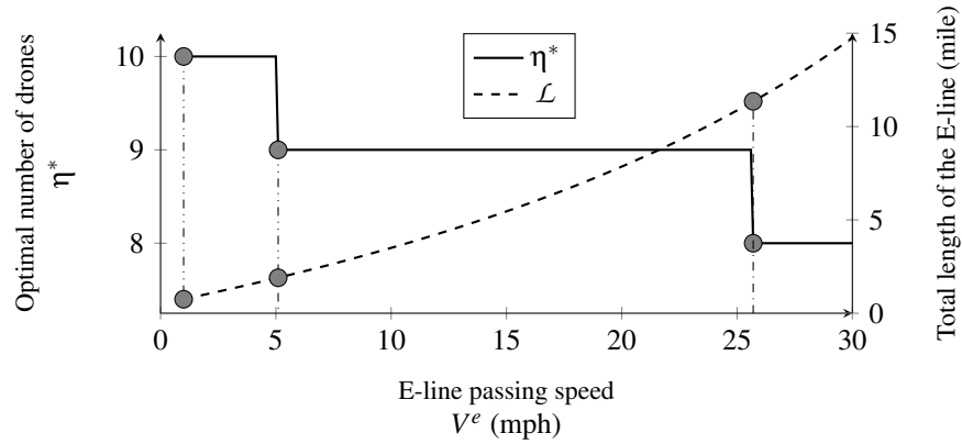
Figure 3: An Example of Optimal Number of Drones and Length of the E-line
