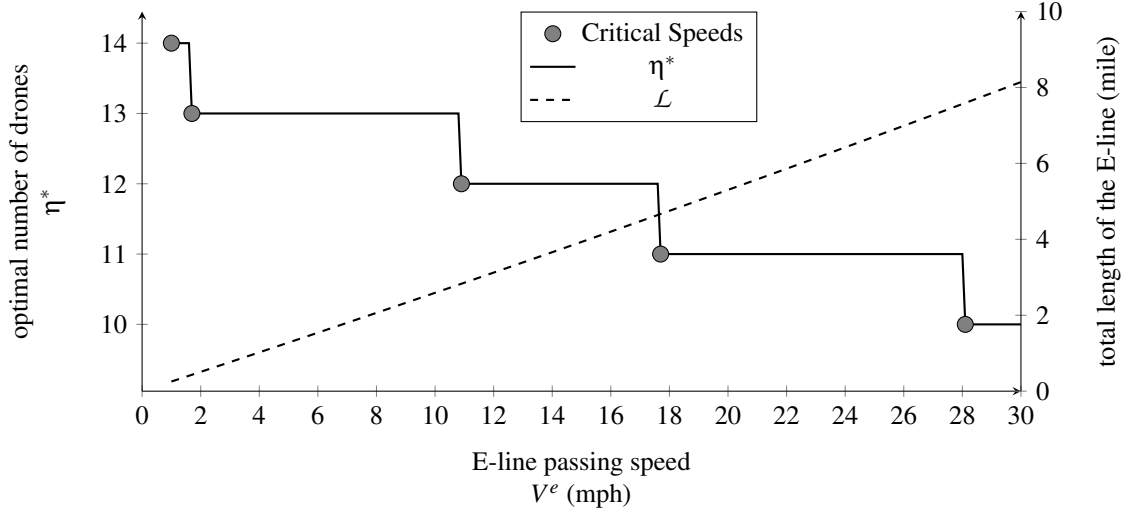
Figure 6: Optimal Number of Drones and Length of the E-line
