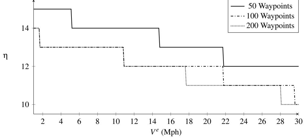
Figure 8: Sensitivity Analysis on changing the number of waypoints
